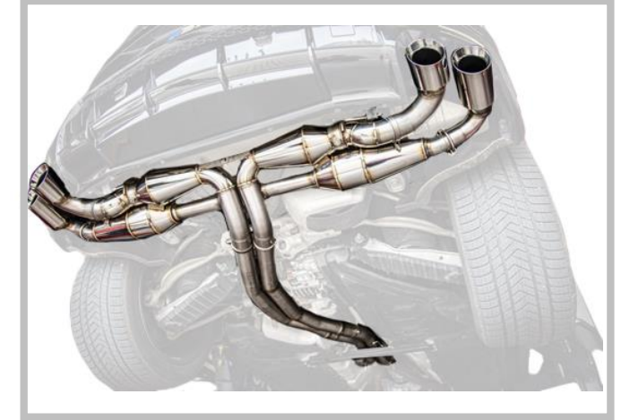
KEYVANY EXHAUST SYSTEM WITH STRAIGHT PIPES + 60 HP
